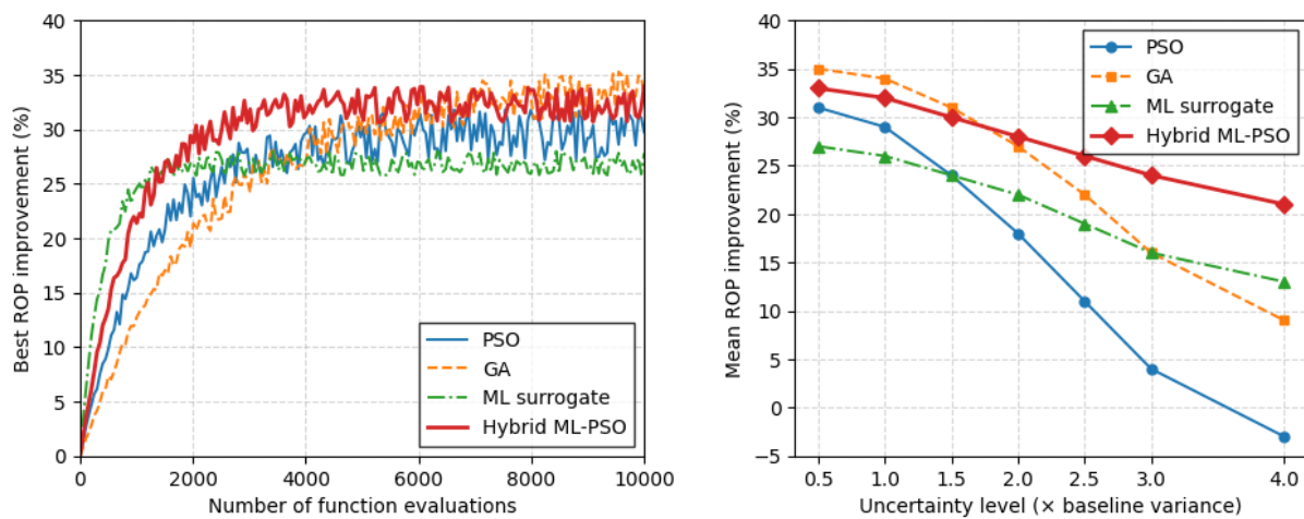
Fig. 1. Convergence curves and robustness comparison of PSO, GA, ML surrogate, and hybrid ML-PSO methods across increasing levels of input uncertainty
