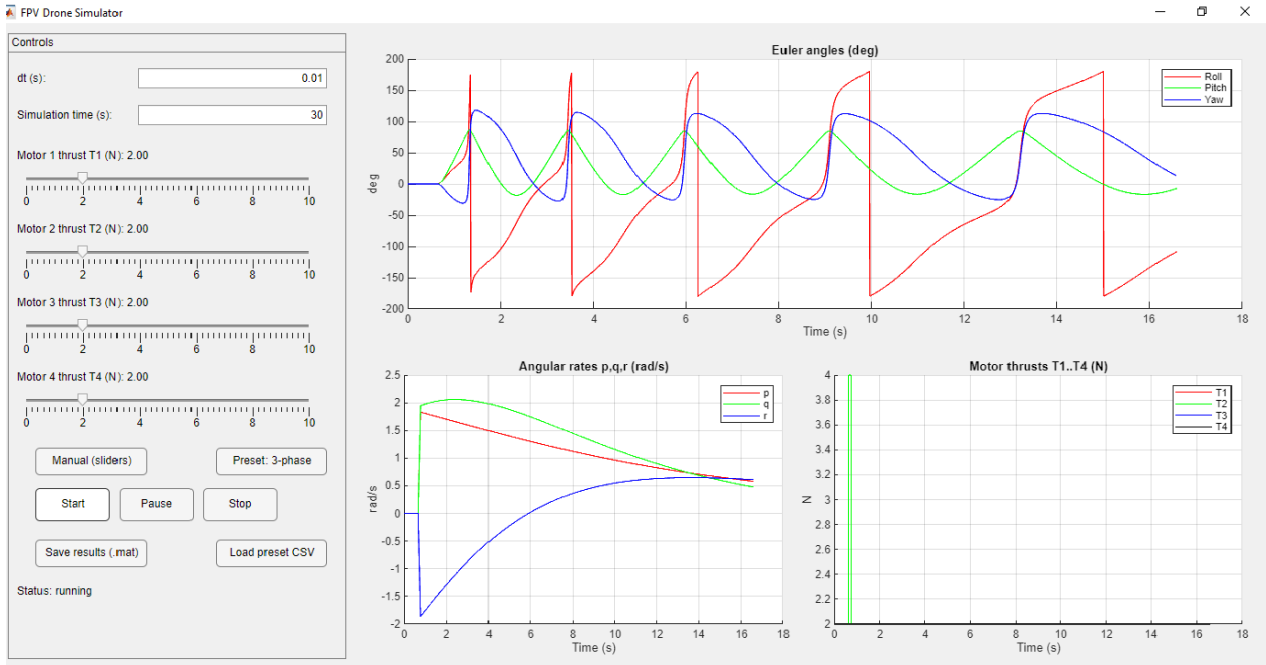
Fig. 1. FPV drone simulation module interface
