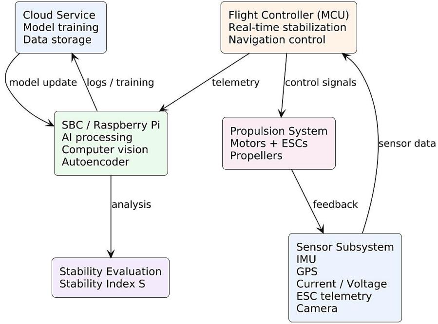
Fig. 1. Simplified architecture of the UAV air segment stability monitoring system with multi-sensor data processing and neural network-based stability evaluation
