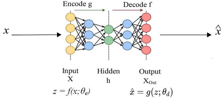
Fig. 3. Autoencoder-based anomaly detection scheme
