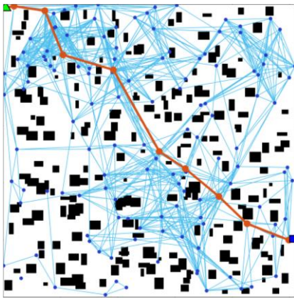
Fig. 6. The path is of 11 nodes
