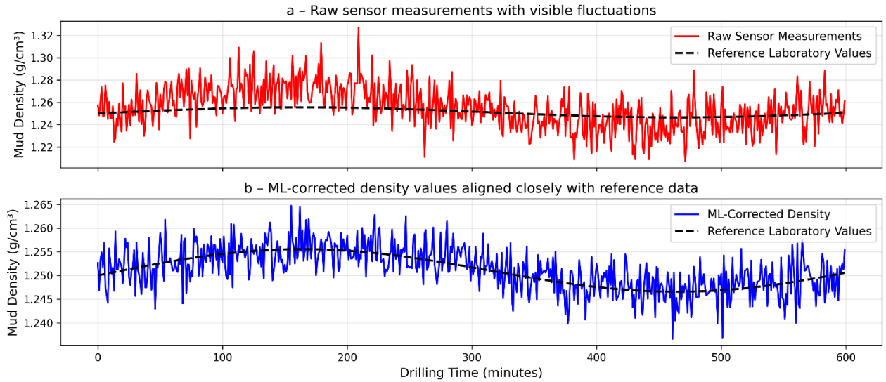
Fig. 1. Comparison of raw measured fluid density versus ML-corrected density over a drilling interval, showing reduced deviation from reference laboratory values. a – Raw sensor measurements with visible fluctuations; b – ML-corrected density values aligned closely with reference data
