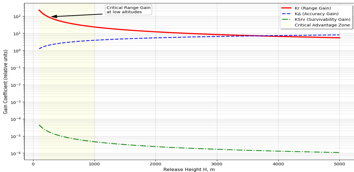
Fig. 2. Dependence of effectiveness gain coefficients on release height
