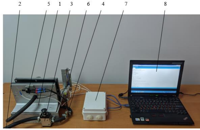
Fig. 1. Automated system of control and data processing equipment for footwear manufacturing
