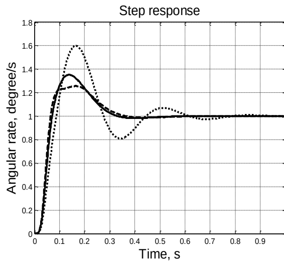
Fig. 2. The transient process on the angular rate for the changed coefficient of rigidity between the shafts of the platform with the equipment and actuator
