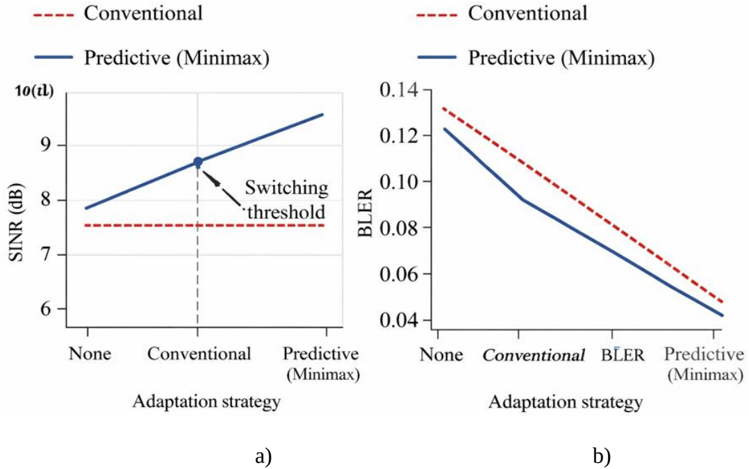
Fig. 1. Performance of adaptive strategies under jamming: (a) SINR versus adaptation strategy; (b) BLER versus adaptation strategy
