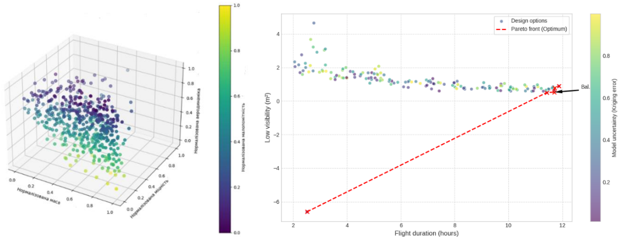
Fig. 1. Visualization of the search for the best design parameters
