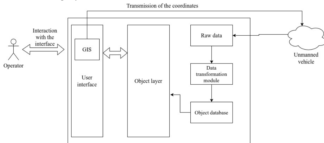
Fig. 1. The structure of the unmanned mission editor
