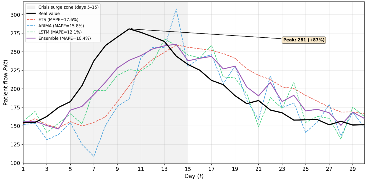
Fig. 1. Dynamics of actual and forecasted workload P_i(t) for a crisis facility (Scenario B, \tau=1 day). Solid line — actual value; dashed lines — forecasts by ETS, ARIMA, LSTM, and the ensemble. The crisis surge zone (days 5–15) is highlighted in gray
