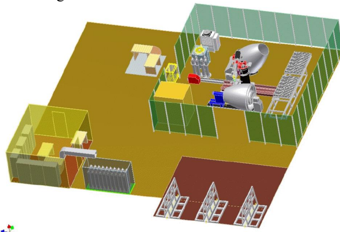
Fig. 1. General view of a model of an automated production system for laser processing of complex profile parts
