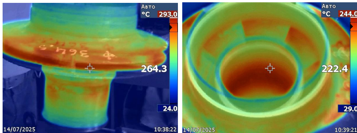
Fig. 2. Surface temperature measurement results after heating
