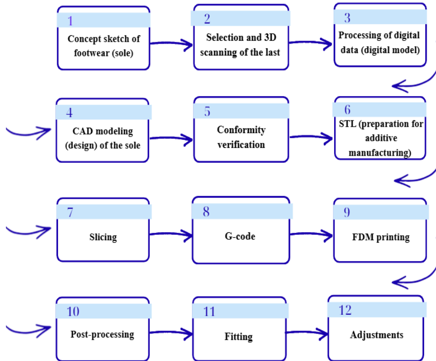
Fig. 1. System for digital design and additive manufacturing of shoe soles
