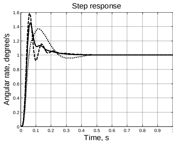
Fig. 1. The transient process on the angular rate for the changed inertia moment of the platform with the equipment
