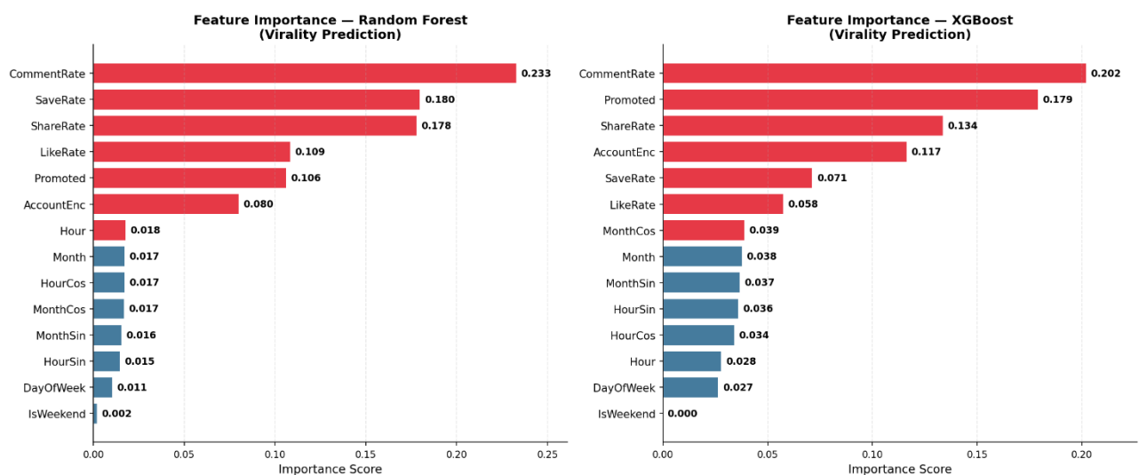
Fig. 2. Feature importance scores for Random Forest and XGBoost classifiers
