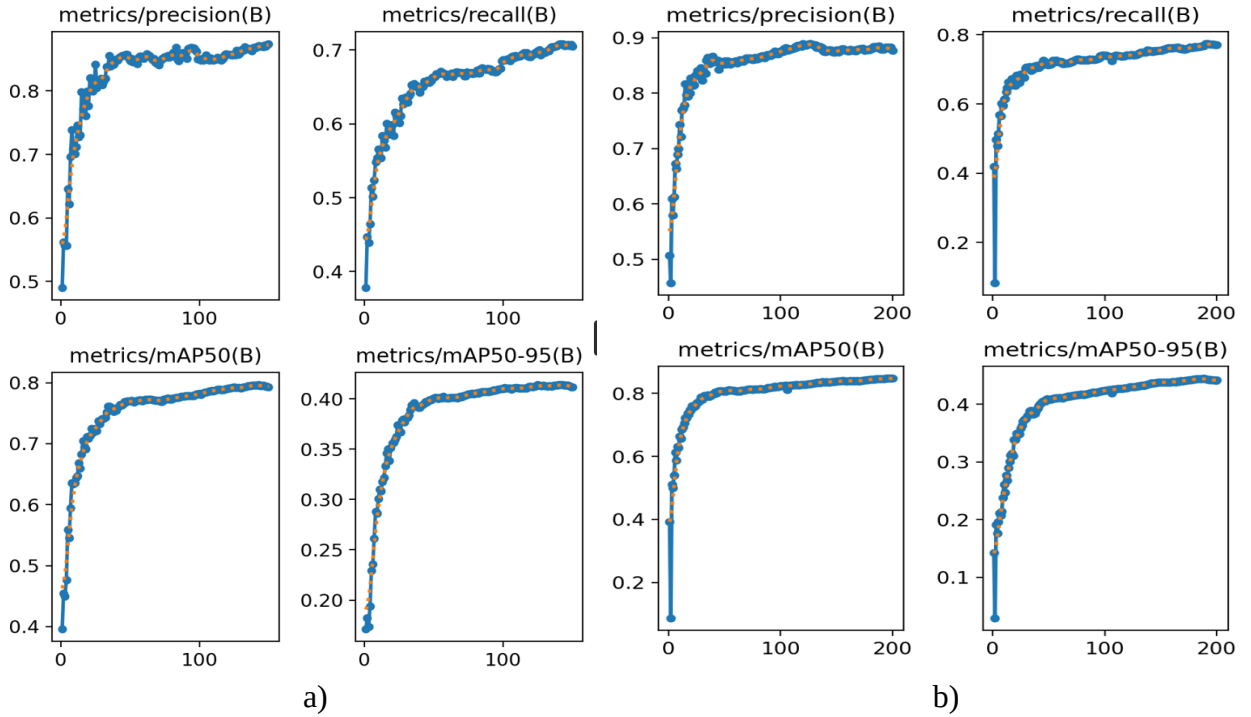
Fig. 1. Comparative characteristics of accuracy and completeness metrics of YOLOv8 (a) and YOLOv11 (b) models
