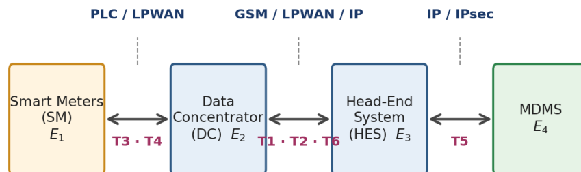
Smart Meter Infrastructure (AMI) — Critical Information Infrastructure
