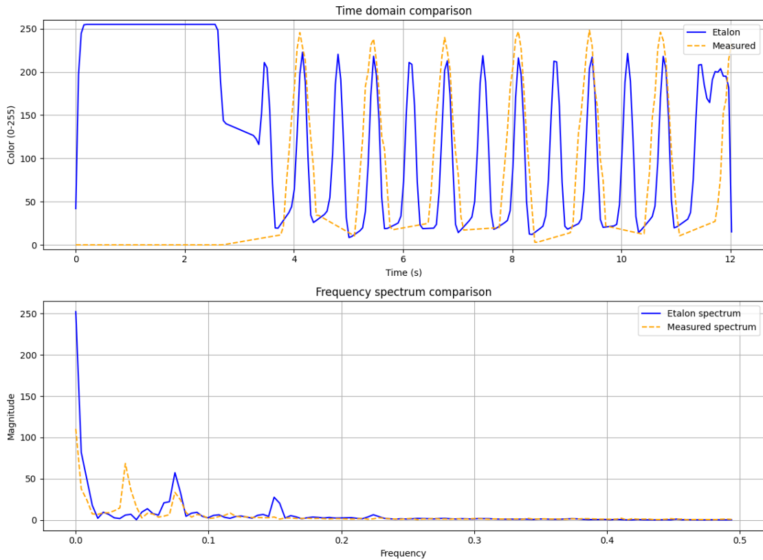
Fig. 2. Comparison of the LED indication reference turn-off pattern (blue) and the defective turn-on pattern measurement (orange), based on R-channel values from the RGB model
