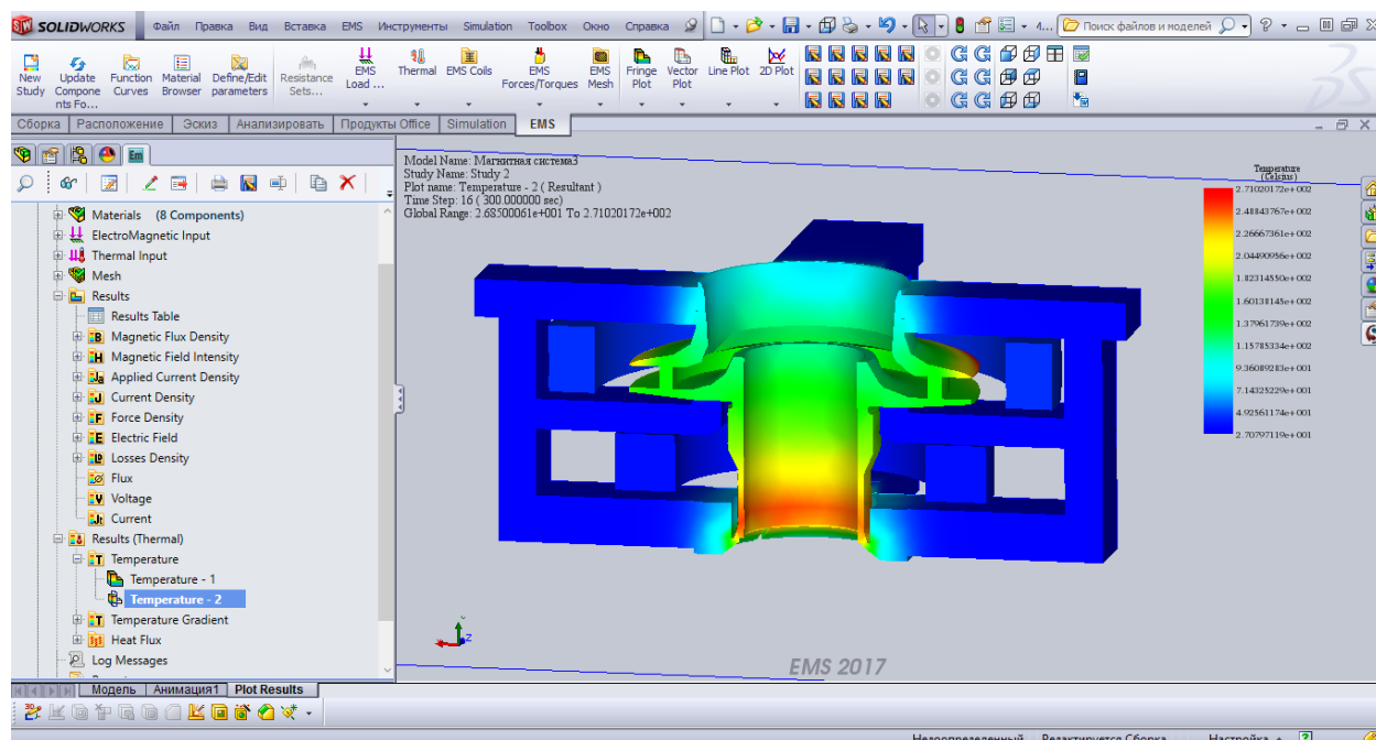
Fig. 1. Axial cross-section of the induction heater and the impeller during simulation
