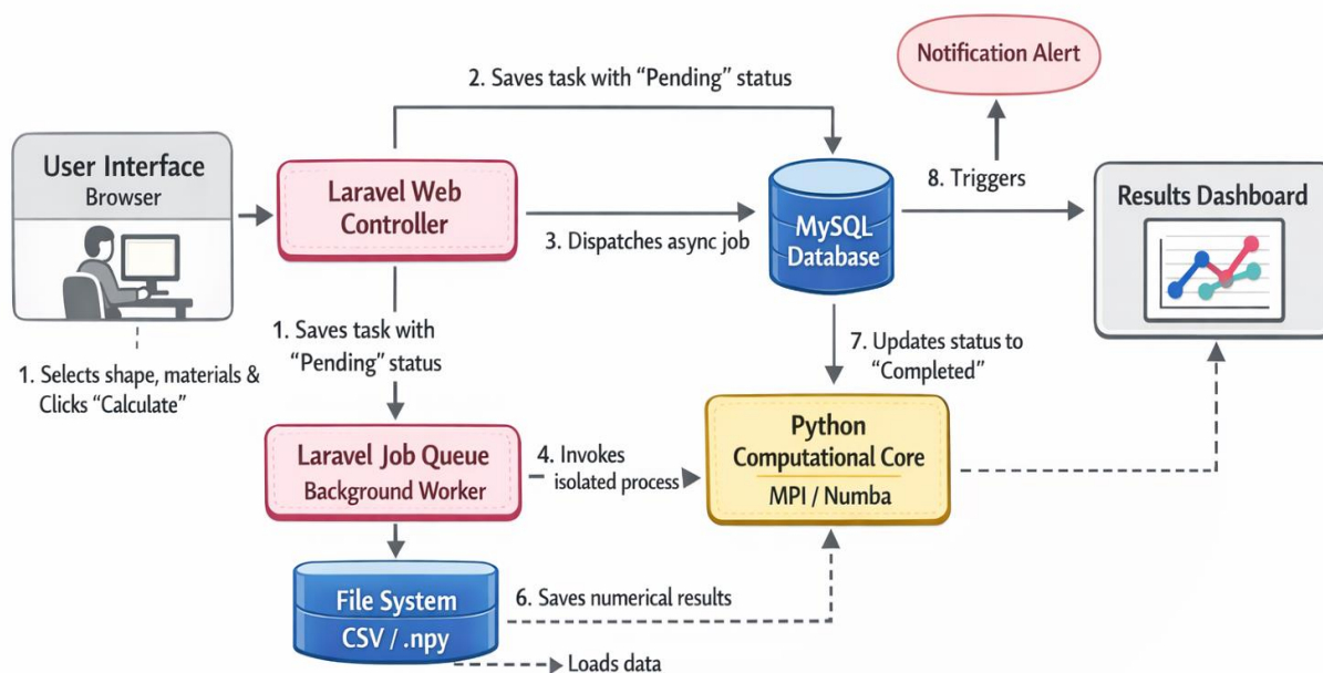
Fig. 1. Block diagram of the hybrid Science Gateway data flow
