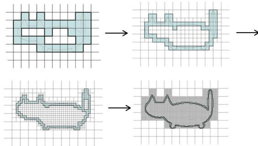
Fig. 2. Variation in the difference between S_k(E) and s_k(E) for the set E , where S_k(E) is the sum of the areas of the squares that contain or intersect E , and s_k(E) is the sum of the areas of the squares entirely contained within the set E
