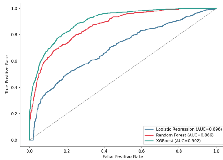
Fig. 1. ROC curves of the virality prediction model
