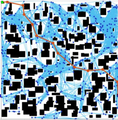
Fig. 7. The path is of 14 nodes
