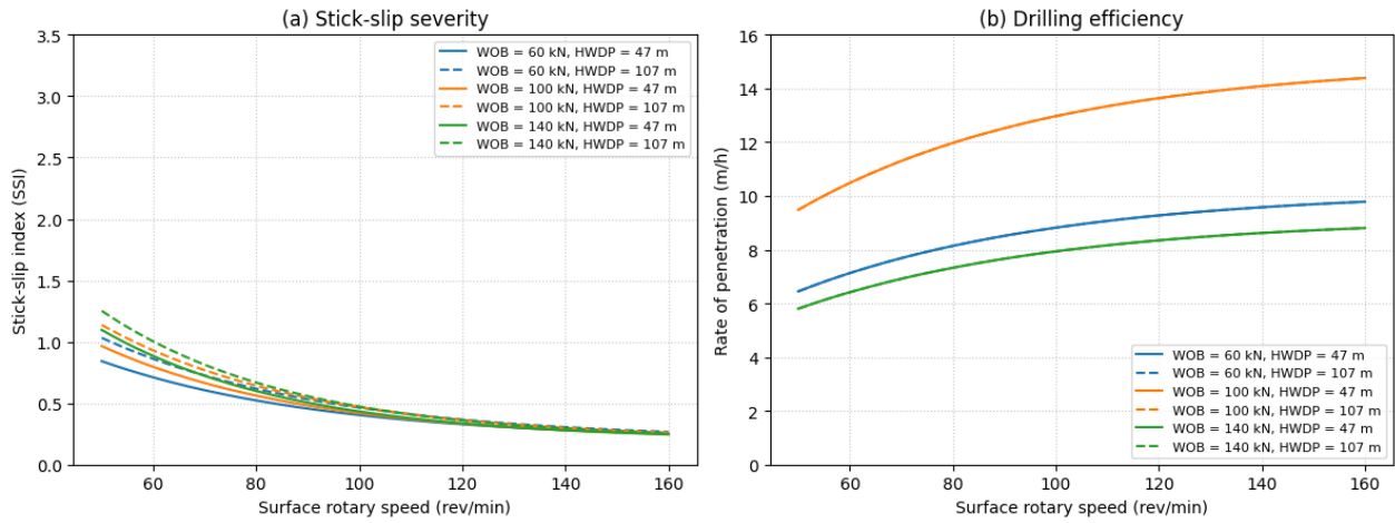
Fig. 1. Stick-slip index (SSI) (a) and rate of penetration (ROP) (b) versus surface rotary speed for different WOB levels (60, 100, 140 kN) and HWDP lengths (47 m baseline vs 107 m), granite-like formation, Herschel-Bulkley fluid with n = 0.75
