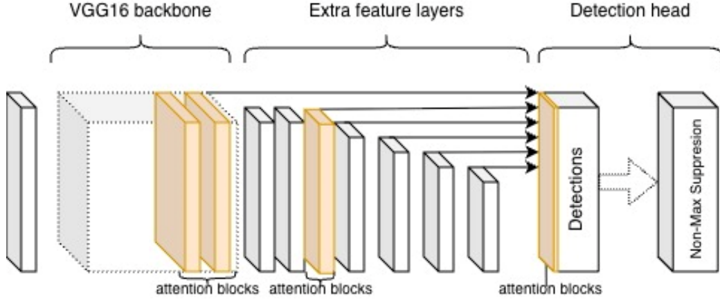
Fig. 2. Attention module placement in SSD300-VGG16
