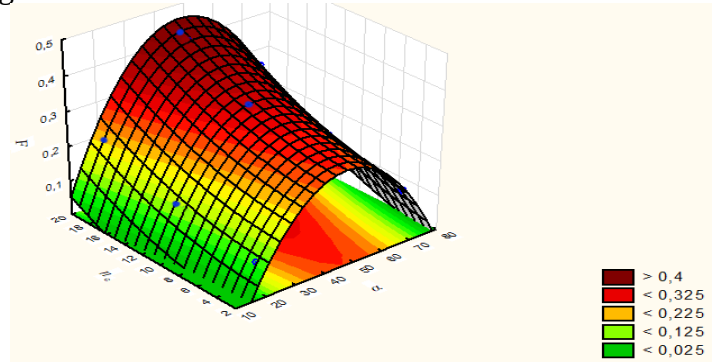
Fig. 2. Graphical dependence of the displacement force response function F=f(\alpha, n_c) at the angle of inclination of the nozzles \alpha and the number of nozzles in each chamber n_c
