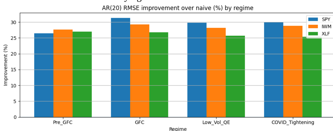
Fig. 3. AR(20) RMSE improvement over naive by regimes and assets
