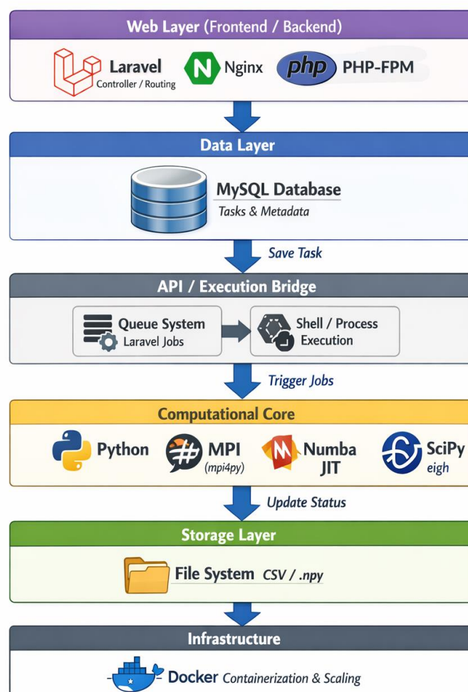
Fig. 2. The technology stack
