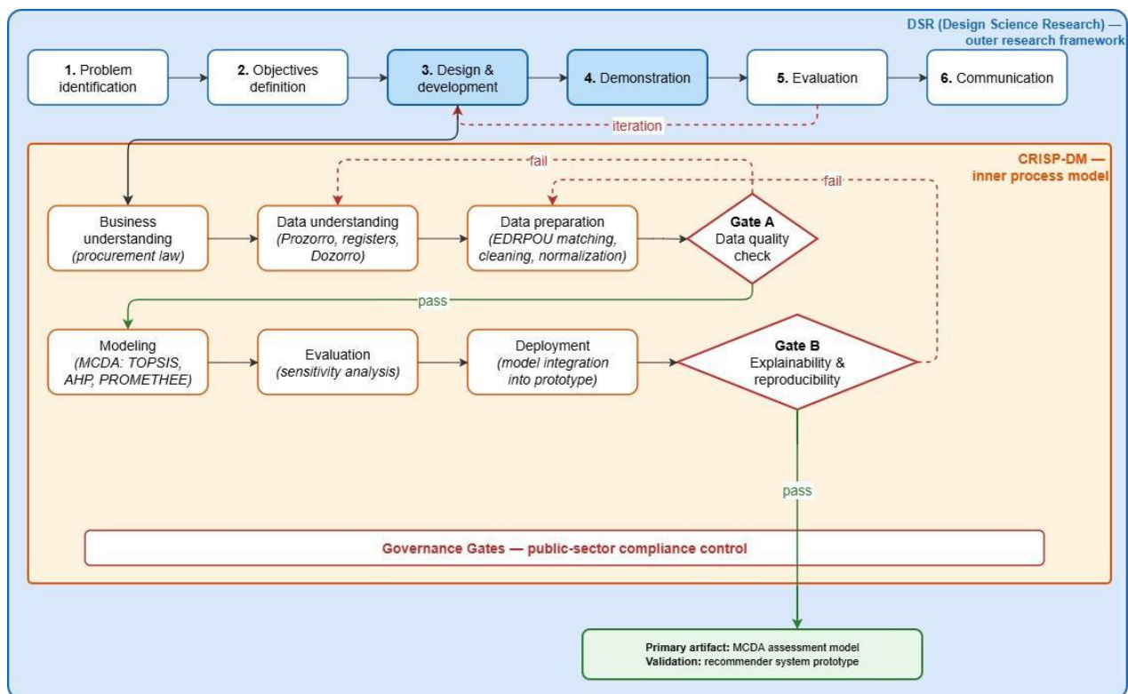
Fig. 1. Structure of the hybrid DSR-CRISP-Gov approach
