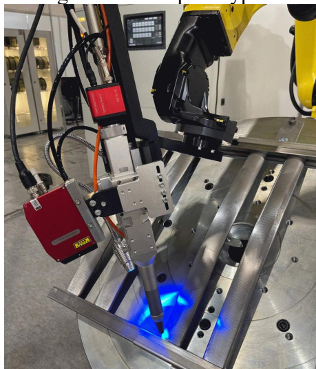
Fig. 2. Prototype automated laser processing system for processing of components with complex profiles
