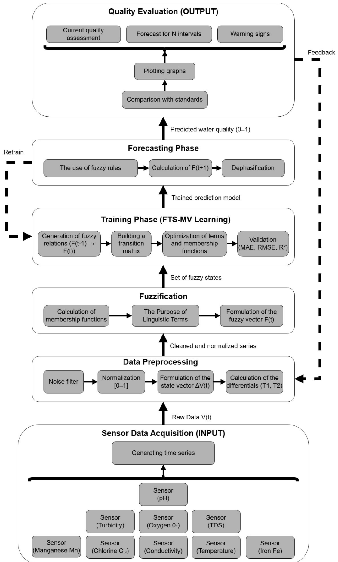
Fig. 1. General architecture of the data processing pipeline of the intelligent monitoring system
