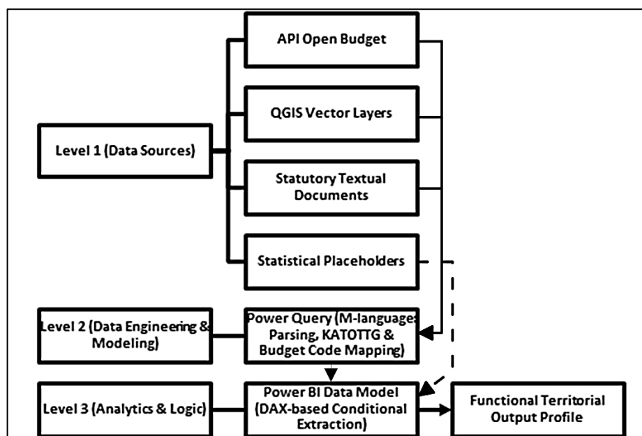
Fig. 1. System architecture and data flow diagram of the territorial classification framework
