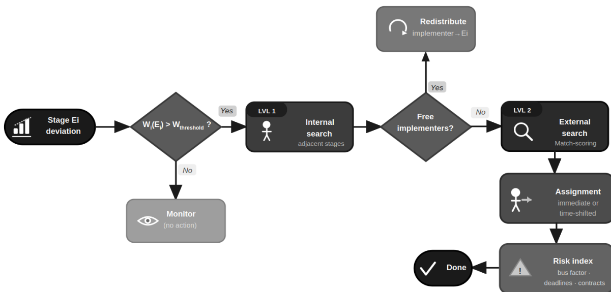
Fig. 1. Two-level load balancing strategy for collaborative project implementers
