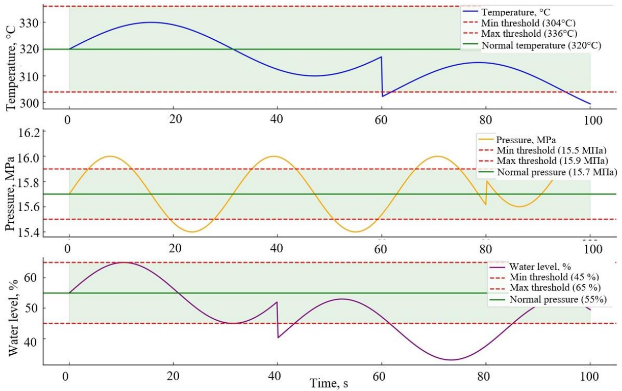
Fig. 2. Schedule of changes in technological parameters in the first circuit of the NPP power unit
