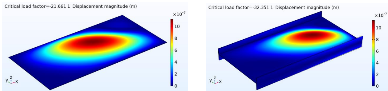
Fig. 1. Comparison of stress-strain states in a simply supported plate and a plate with elastically supported long edges
