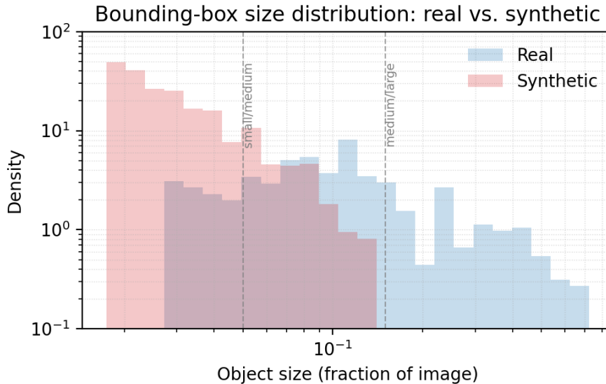
Fig. 3. Distribution of UAV bounding-box sizes in real and synthetic images
