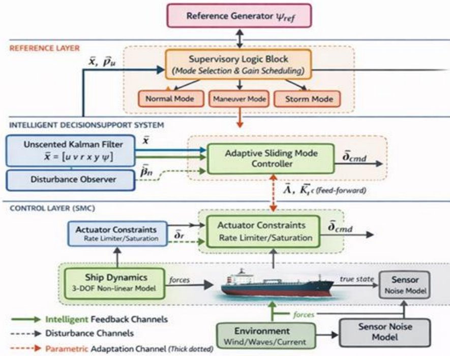
Fig. 1. Structural-functional diagram for ISM implementation in the MATLAB/Simulink environment
