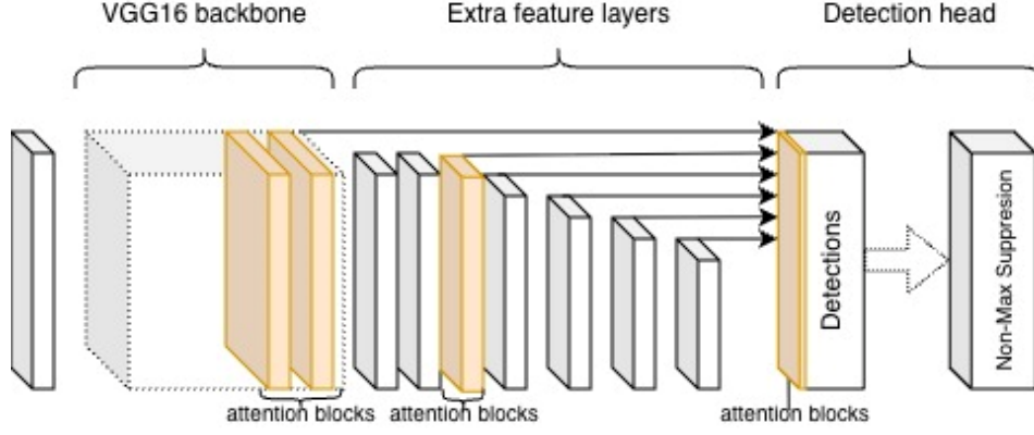
Fig. 1. Attention module placement in SSD300-VGG16
