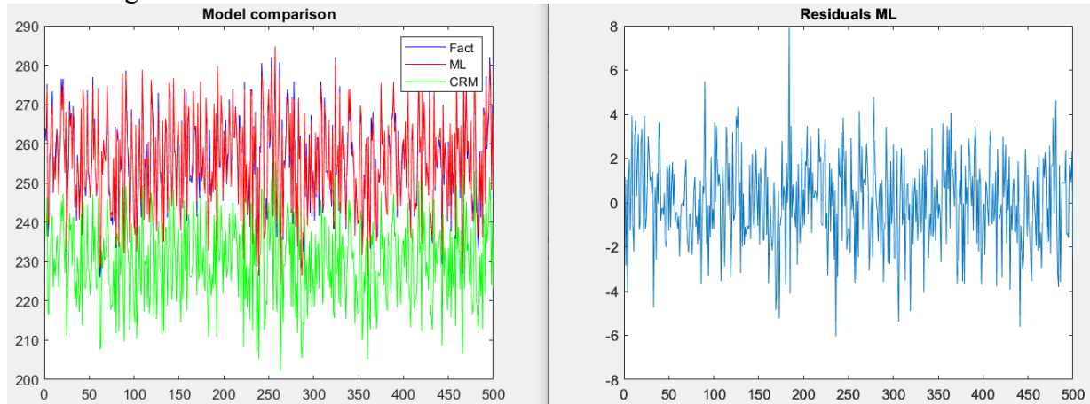
Fig. 2. Comparison of pellet price formation using the operational CRM model (CRM) and using the supplementary analytical module (ML), and the error between ML and the actual price value (Fact)
