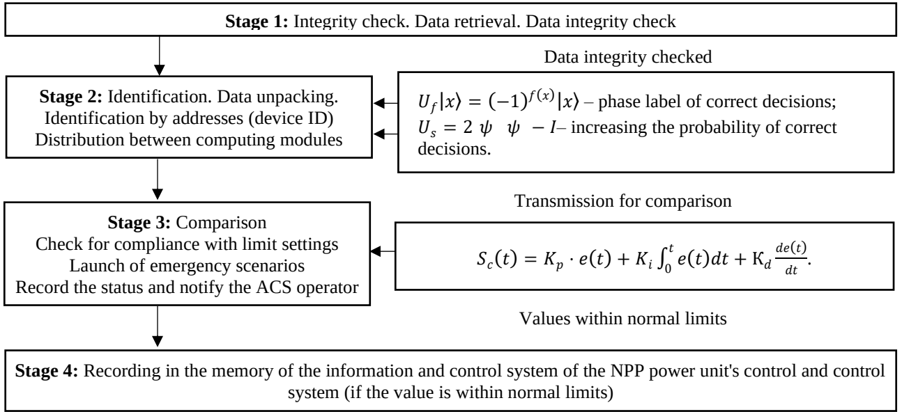
Fig. 1. Structure diagram of the sequence of stages of parallel data processing in the central node of the microprocessor
