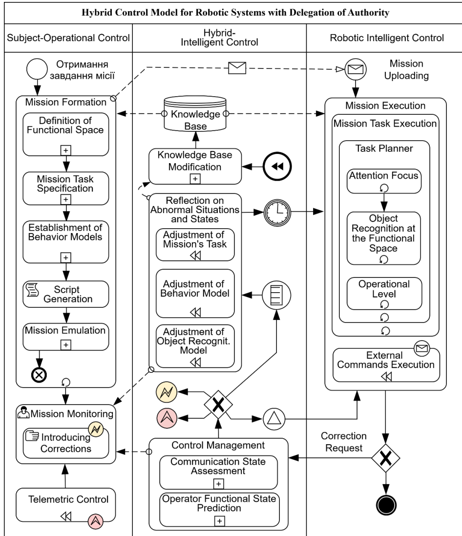
Fig. 1. Hybrid Control Model for Robotic Systems with Delegation of Authority
