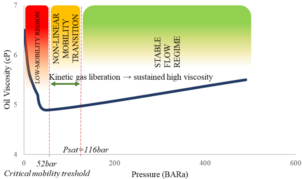
Fig. 1. Kinetic gas liberation delay demonstrating anomalous viscosity retention below the saturation pressure
