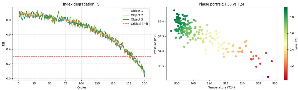
Fig. 2. Results of monitoring the functional stability of the HPS energy system
