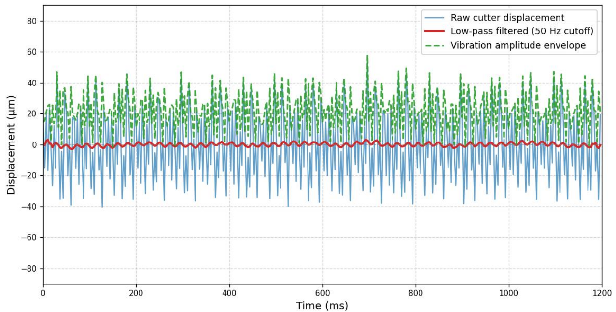
Fig. 1. Measured cutter vibration amplitude versus time showing periodic oscillations at dominant frequencies of 120–280 Hz
