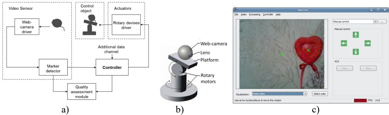
Fig. 1. Structure and some components of the research complex
