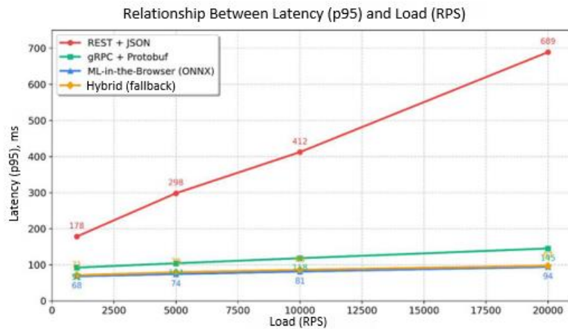
Fig. 1. Latency-RPS Chart
