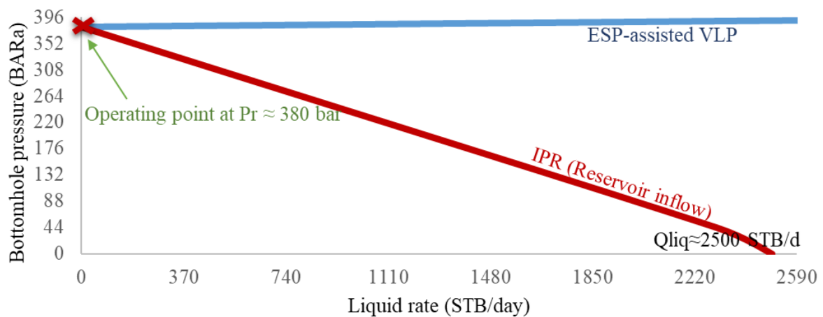
Fig. 2. Nodal analysis illustrating a stabilized operating point achieved through ESP integration
