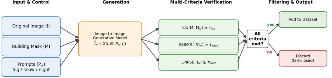
Fig. 1. General scheme of the topology-preserving weather augmentation method
